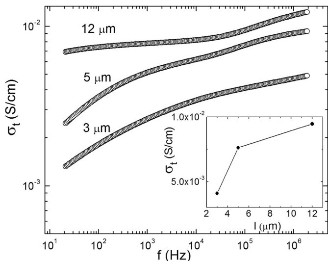
Fig. 3. Frequency dependences of total electrical conductivity at T = 298 K for (\text{Cu}_{0.5}\text{Ag}_{0.5})_7\text{Si}_5\text{I} ceramic samples with different sizes of crystallites: 12 \mu\text{m} , 5 \mu\text{m} , and 3 \mu\text{m} . The insert shows the dependence of the total electrical conductivity on the size of crystallites at 100 kHz.
