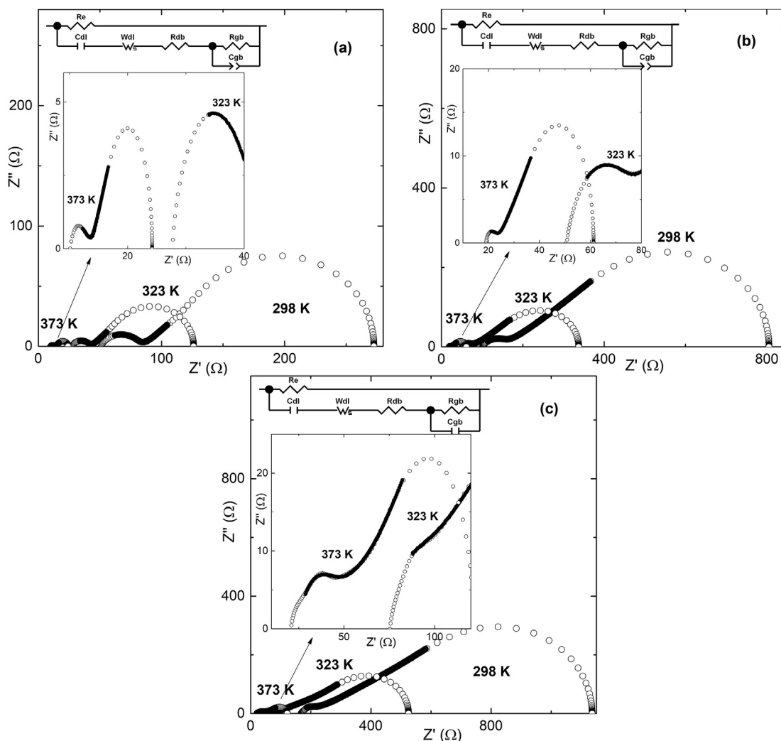
Fig. 4. EEC and Nyquist plots for (\text{Cu}_{0.5}\text{Ag}_{0.5})_7\text{Si}_5\text{I} ceramic samples with different crystallite sizes: (a) 12 \mu\text{m} ; (b) 5 \mu\text{m} ; (c) 3 \mu\text{m} for different temperatures. Experimental data correspond to the solid dots, calculated data correspond to the open dots.
