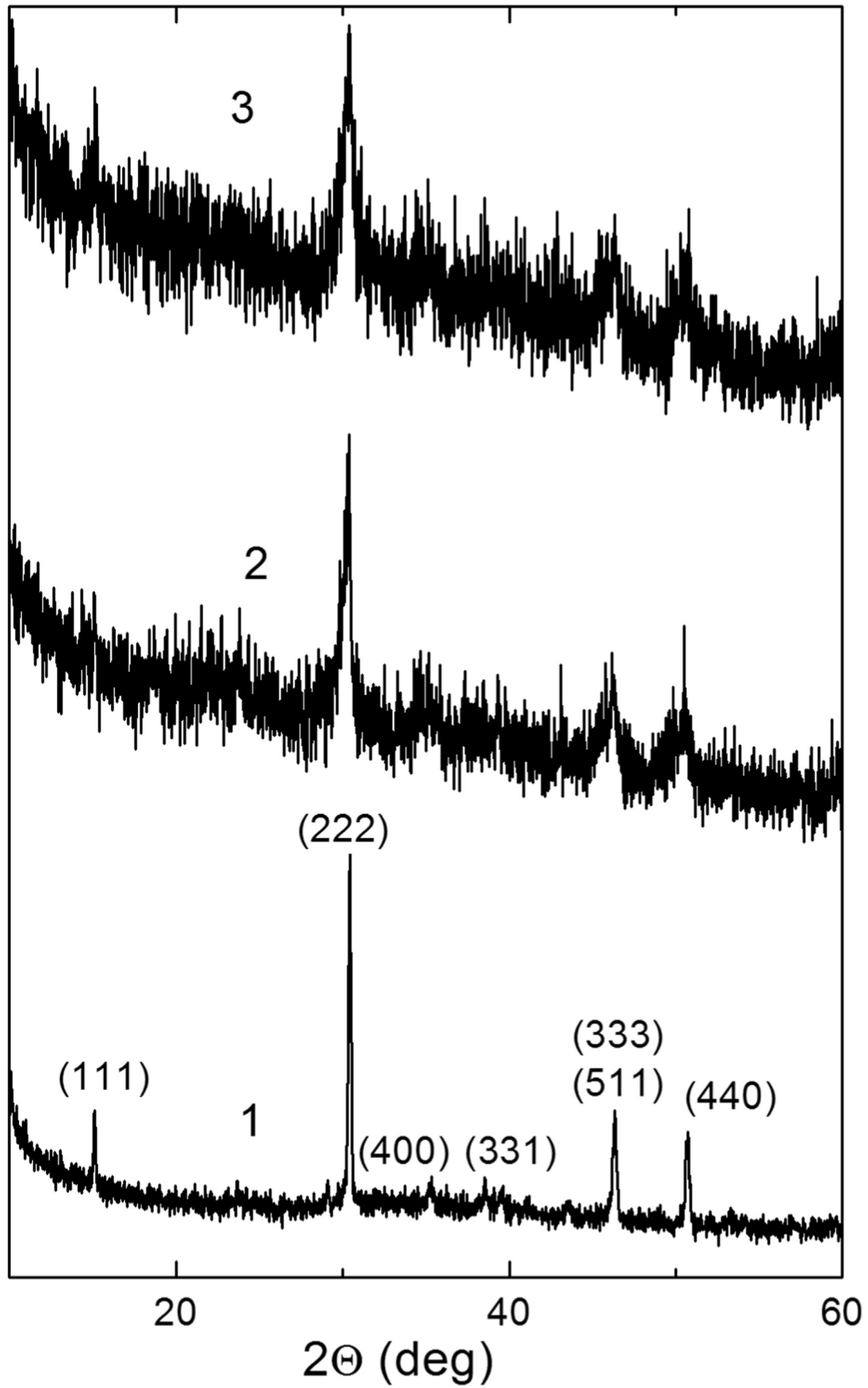
Fig. 1. Diffractograms of (\text{Cu}_{0.5}\text{Ag}_{0.5})_7\text{Si}_5\text{I} powders obtained by grinding in agate mortar (1) and planetary ball mill for 30 min (2) and 60 min (3).
