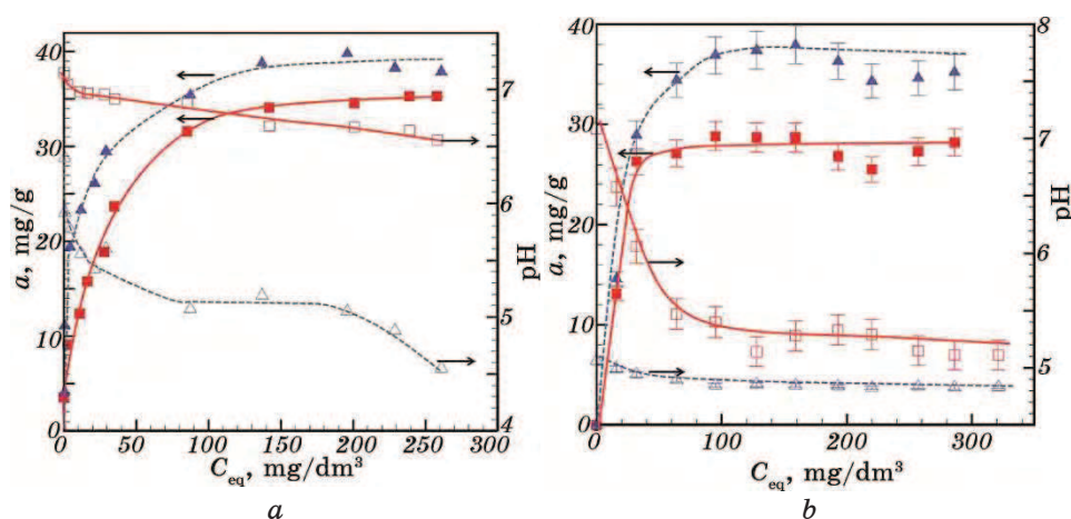
Fig. 6. Adsorption isotherms of the Ni(II) (a) and Cu(II) (b) ions by the as-prepared (squares) and oxidized (triangles) N-CNTs at ‘natural’ pH of the suspension (pH 5.0–6.0). In addition, the changes in the equilibrium pH of a 0.1% suspension because of ions’ adsorption are also shown.
